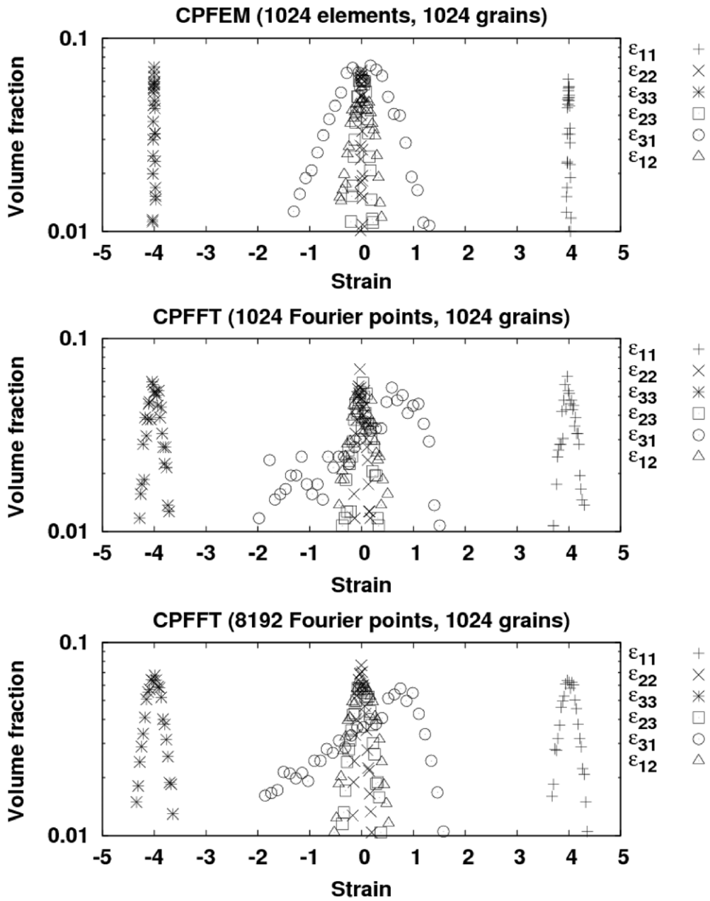
Figure 7. Strain distributions after plane-strain compression at 98% thickness reduction: CPFEM with periodic boundary conditions (1024 elements, 1024 grains), CPFFT (1024 Fourier points, 1024 grains), CPFFT (8192 Fourier points, 1024 grains).
