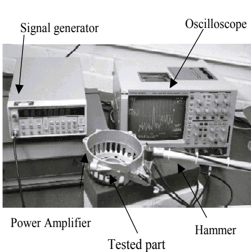
FIGURE 3. Experimental setup for alternator housing test
