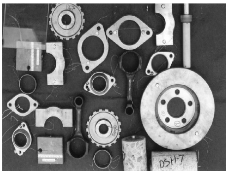
FIGURE 5. A number of tested parts.
