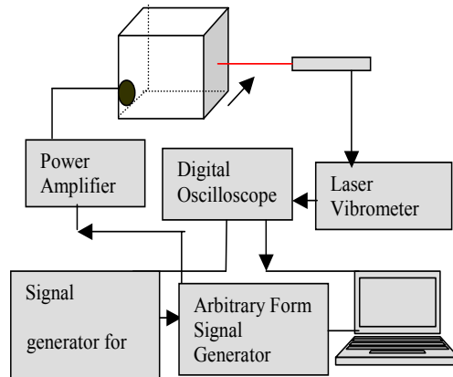
FIGURE 8. The experimental setup for TRA focusing in a glass parallelepiped sample.
