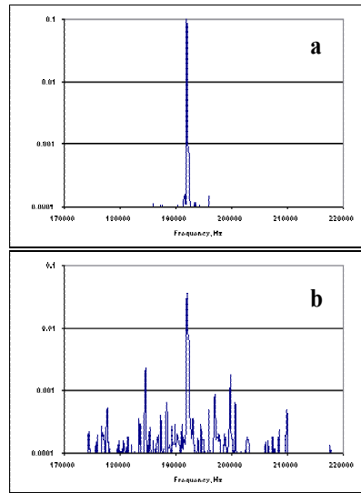
FIGURE 4. Spectra of the received signal for a) the intact sample, and b) the sample with a tiny crack.
