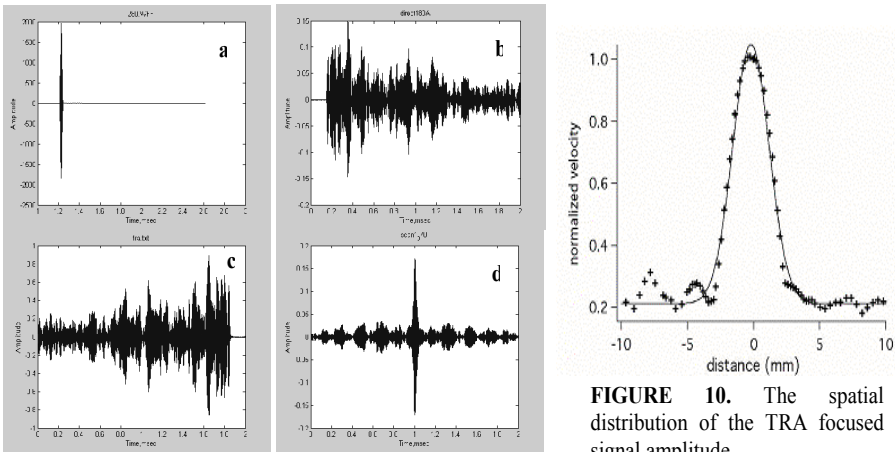
FIGURE 9. TRA focusing in the glass: a) initial radiated in Step 1 r.f. signal, b) direct recorded signal of Step 2, c) radiated TR signal, d) detected focused TR signal.
