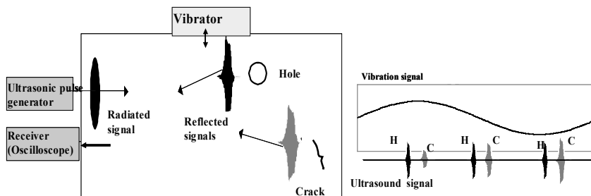
FIGURE 6. Concept of a pulse modulation method.
