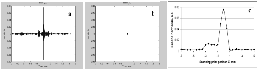
FIGURE 11. The TRA focused signal filtered around second harmonics (520 kHz): a) signal on the surface above the crack, b) signal on an intact surface, c) spatial distribution of the second harmonic amplitude along the sample surface.
