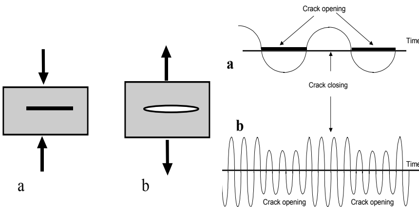
FIGURE 1. Sample with flaw: a - closed by vibration compression, b - open under dilation.
