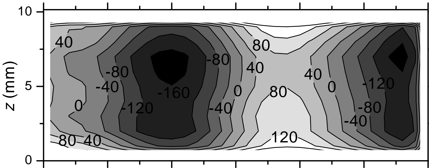
b. Uncorrected contour results.
