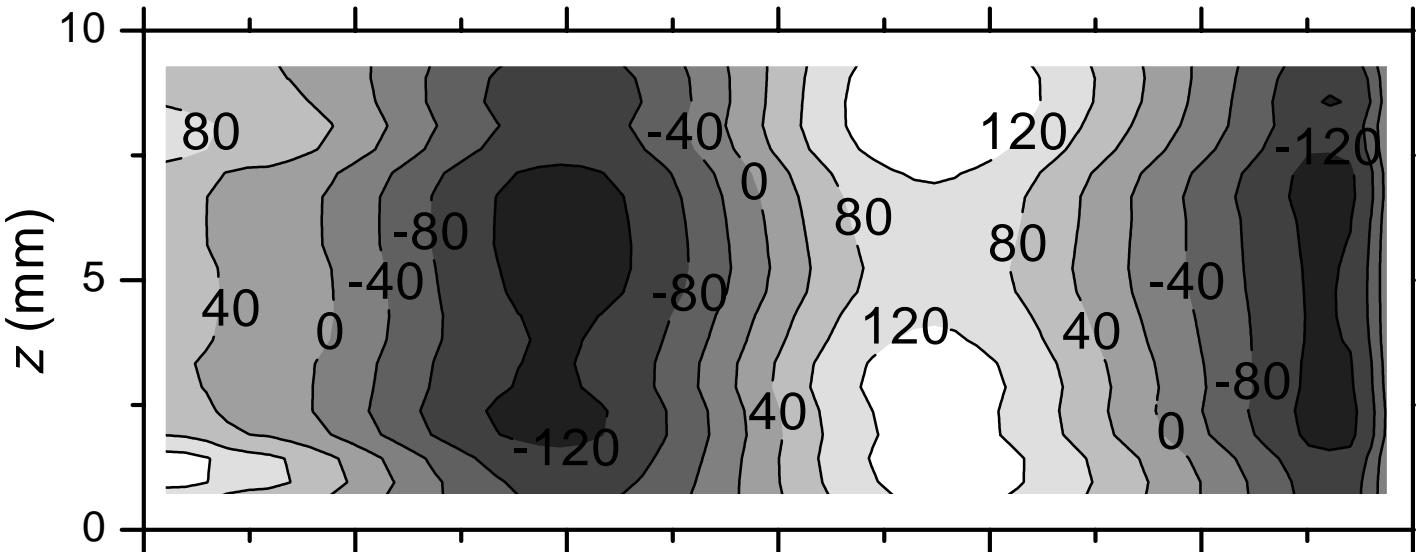
c. Corrected contour results.
