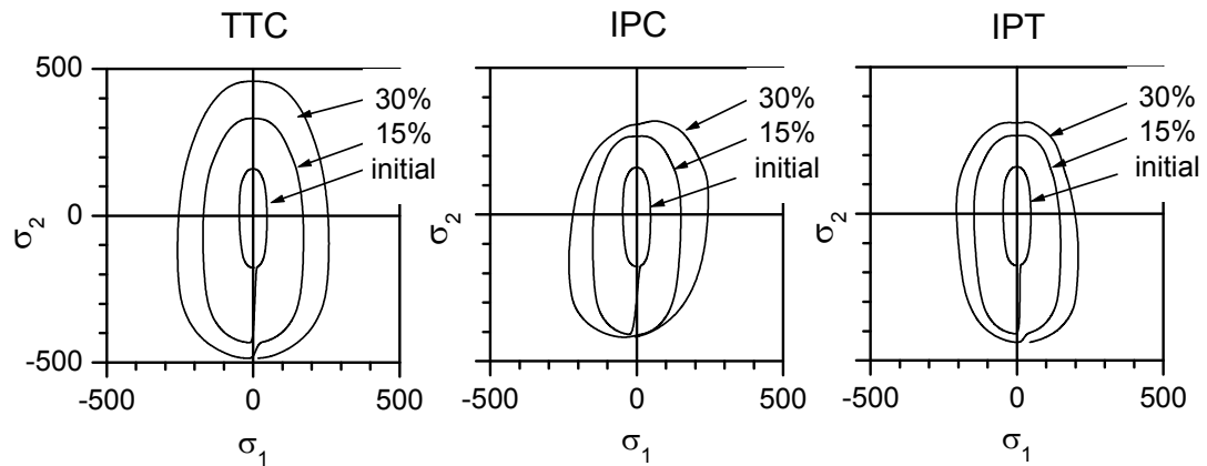
Figure 7-3: Polycrystal Yield Surface ( \pi -plane projection) for Zr deforming in TTC, IPC and IPT. Intermediate projections calculated at 0%, 15% and 30% strain. Observe that the PCYS is not centro-symmetric due to the presence of tensile twinning. The increase in shape with deformation is associated with hardening. The shape distortion for the IPC case is associated with twinning reorientation.
