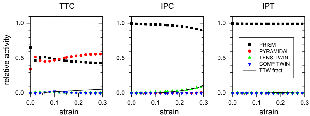
Figure 7-4: Relative contribution of prism slip, pyramidal slip and tensile twins to deformation for clock-rolled Zr, deforming at room temperature in Through Thickness Compression, In-Plane Compression and In-Plane Tension. Also shown is the volume fraction of twinned material as a function of strain. Although Compressive twinning is included in the calculation it does not contribute to deformation at room temperature.
