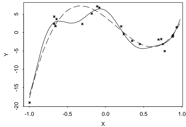
9-th degree
