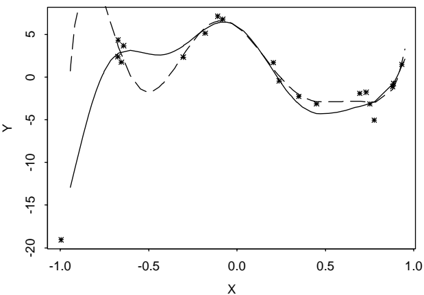
13-th degree
