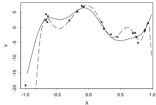
17-th degree
