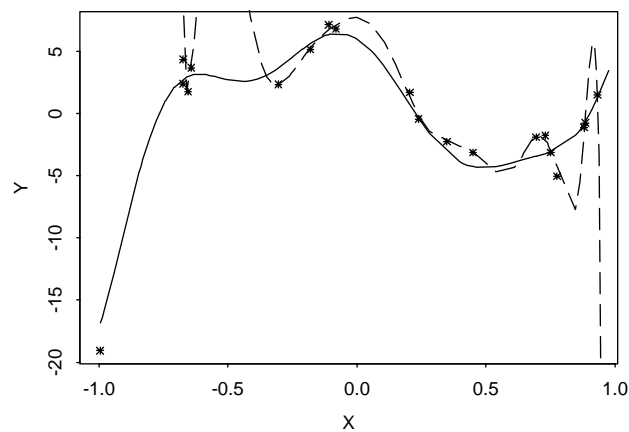
15-th degree
