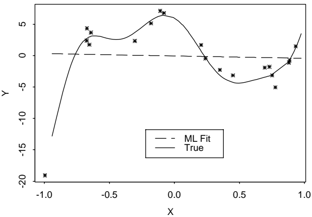
7-th degree
