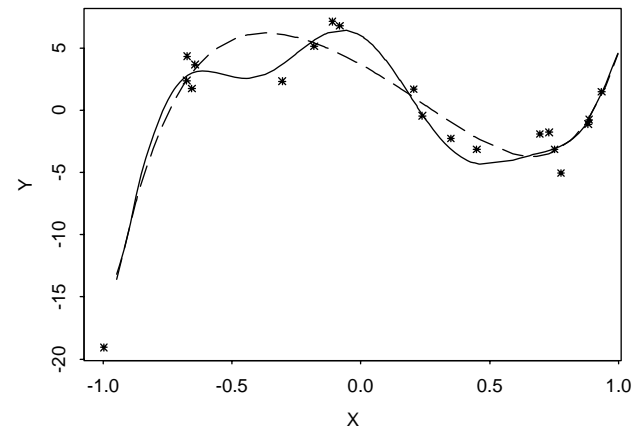
11-th degree
