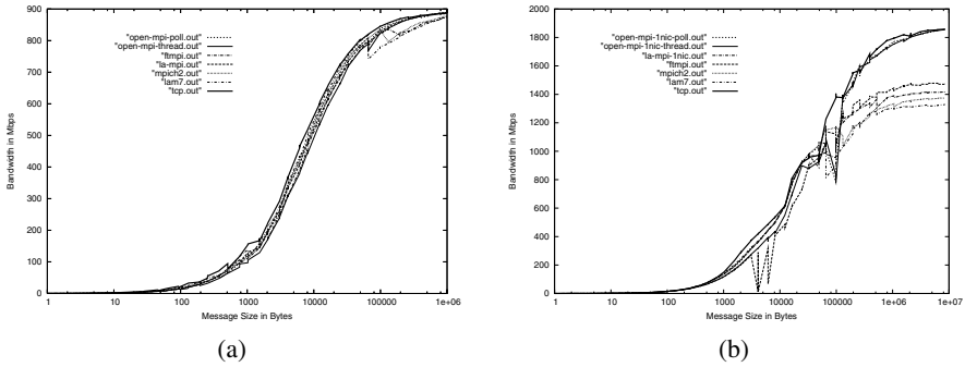
Fig. 1. Open MPI/TEG point-to-point ping-pong bandwidth compared to with the MPICH2, FT-MPI, LA-MPI, and LAM/MPI implementations, and raw TCP/IP. (a) Gigabit Ethernet (b) Myrinet.
