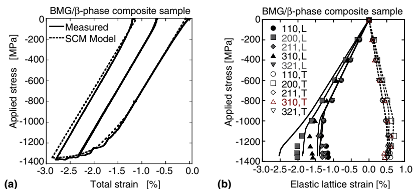
Fig. 2. (a) Comparison of measured (by extensometer) and calculated (SCM) macroscopic stress–strain curve for the composite sample. (b) Comparison of measured (symbols) and calculated (lines) lattice specific stress–strain curves for the \beta phase in the composite sample (“L” and “T” indicate longitudinal and transverse directions, respectively).
