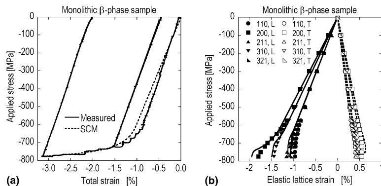
Fig. 1. Measured and calculated response of the monolithic \beta phase sample to applied compressive stress: (a) macroscopic strain along the loading axis; and (b) lattice plane specific elastic strain (symbols designate neutron data while lines are SCM predictions; here “L” and “T” indicate longitudinal and transverse directions, respectively). The difference between measured and calculated macroscopic stiffness shown in (a) is likely due to extensometer problems. This claim is supported by the fact that the diffraction data in the elastic region is in good agreement with the model calculations as shown in (b).
