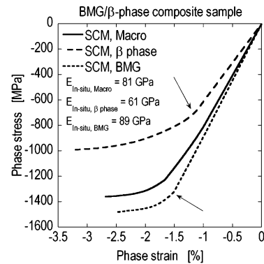
Fig. 3. Calculated in situ behavior (phase stress vs. phase strain) for the composite. The arrows indicate the yield points in the \beta phase (about -650 MPa) and the BMG matrix (around -1350 MPa). The solid line (“macro”) designates the composite behavior. The in situ Young’s moduli for each phase are also shown.
